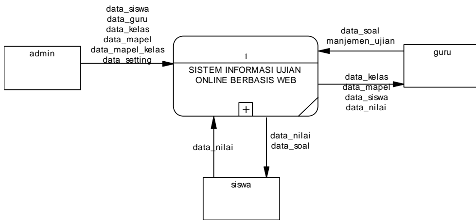
Gambar 3. Context Diagram
