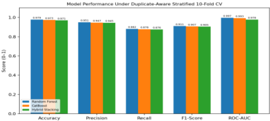
Figure 3. Model comparison under the duplicate-aware protocol.
