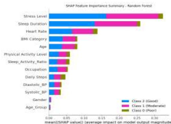
Figure 5. SHAP feature-importance summary for Random Forest.
