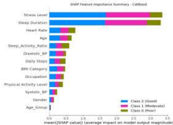
Figure 4. SHAP feature-importance summary for CatBoost.
