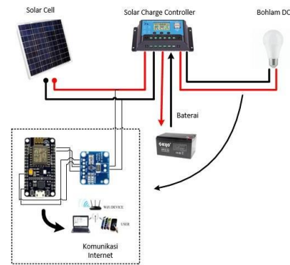
Gambar 1. Diagram Fungsional Sistem
