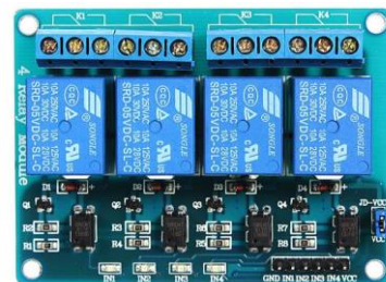
Gambar 9. Modul Relay
