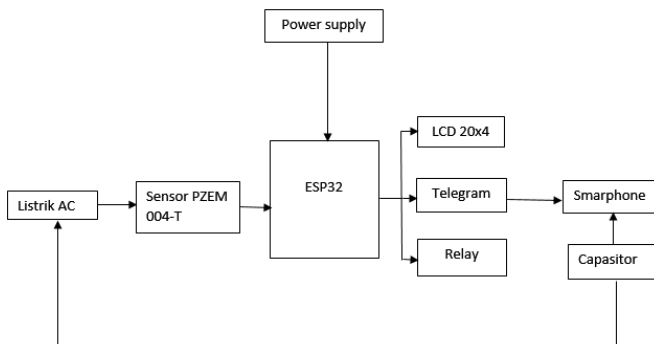
Gambar 3. Block Diagram
