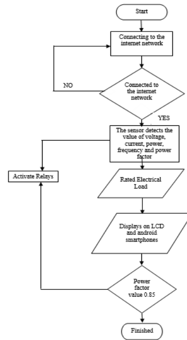
Gambar 4. Flowchart System
